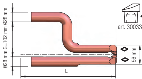
L = 275 mm art. 5271
