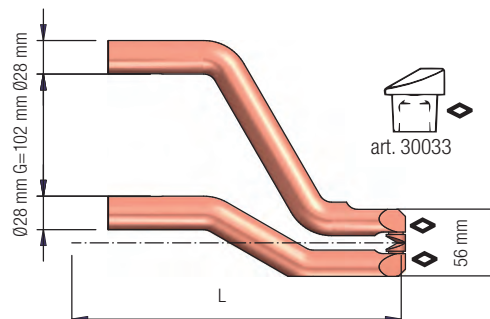
L = 270 mm art. 5272
